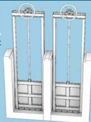
05-010-3L 3 sides sealed penstock
