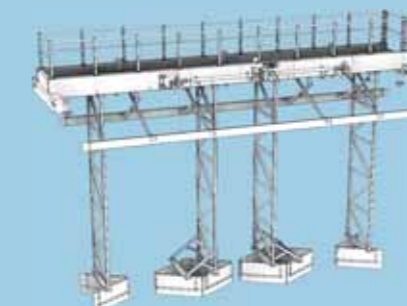
05-078 To & fro sludge suction bridge
