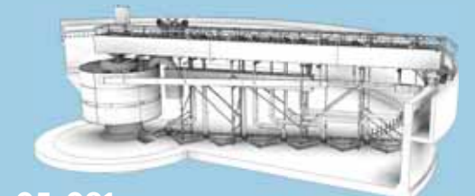
05-091 Peripheral drive sludge suction bridge
