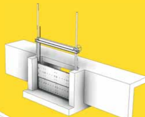
05-010-2B 3 sides sealed penstock double shutter
